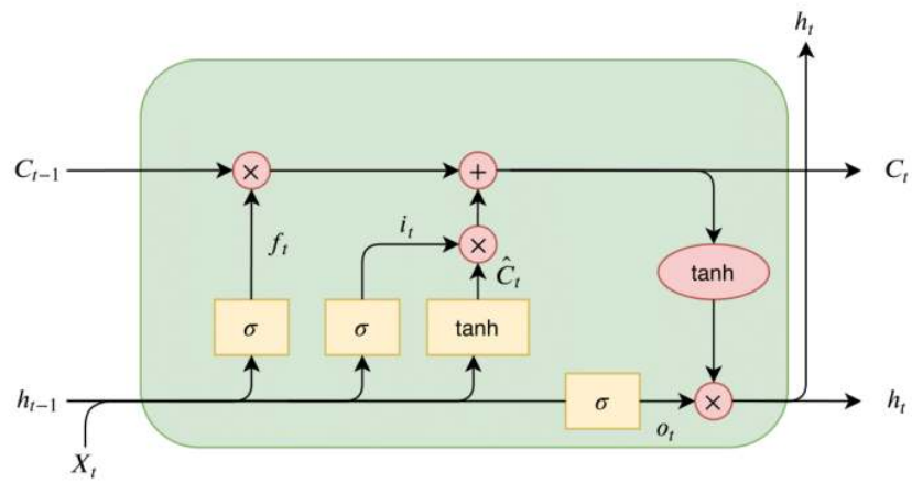
Figure 5.4 LSTM Architecture
