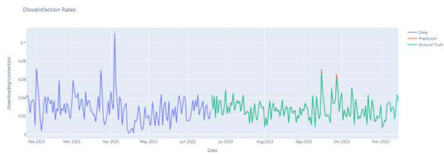
Figure 7.8 Prediction test results for Download/Connectivity
