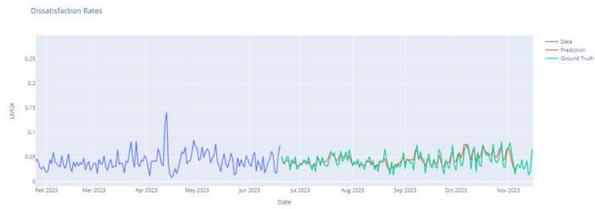
Figure 7.4 Prediction test results for UI/UX
