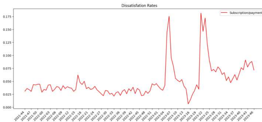
Figure 6.16 Weekly sentiment analysis results for Subscription/Payment
