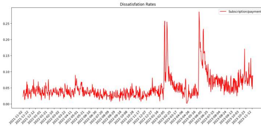
Figure 6.15 Daily sentiment analysis results for Subscription/Payment
