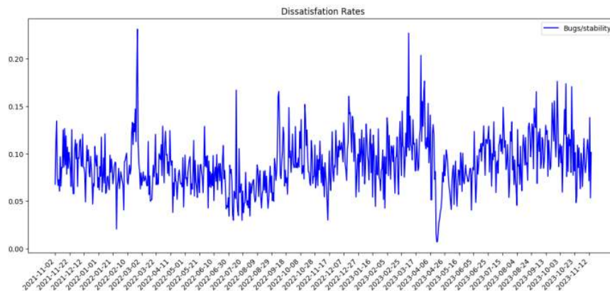
Figure 6.9 Daily sentiment analysis results for Bugs/Stability
