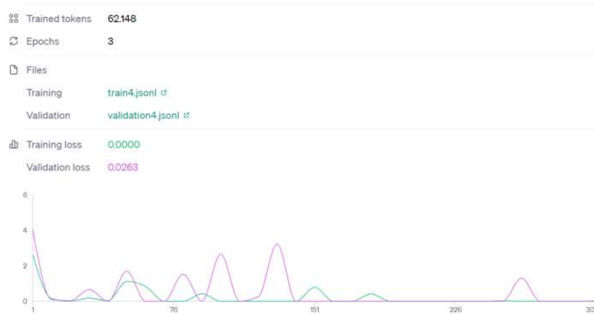
Figure 6.2 GPT-3.5 Turbo 1106 Learning Curve
