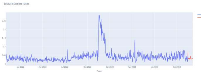
Figure 6.25 UI/UX basis future prediction results
