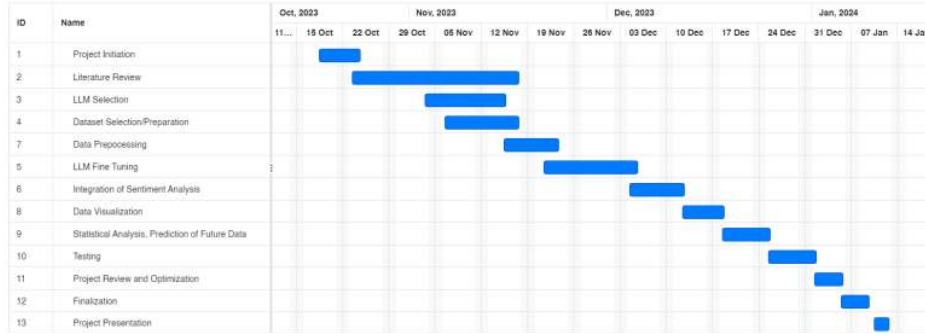
Figure 3.1 Gantt diagram
