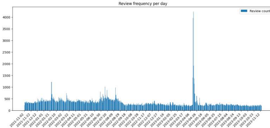
Figure 5.3 Reviews Frequency
