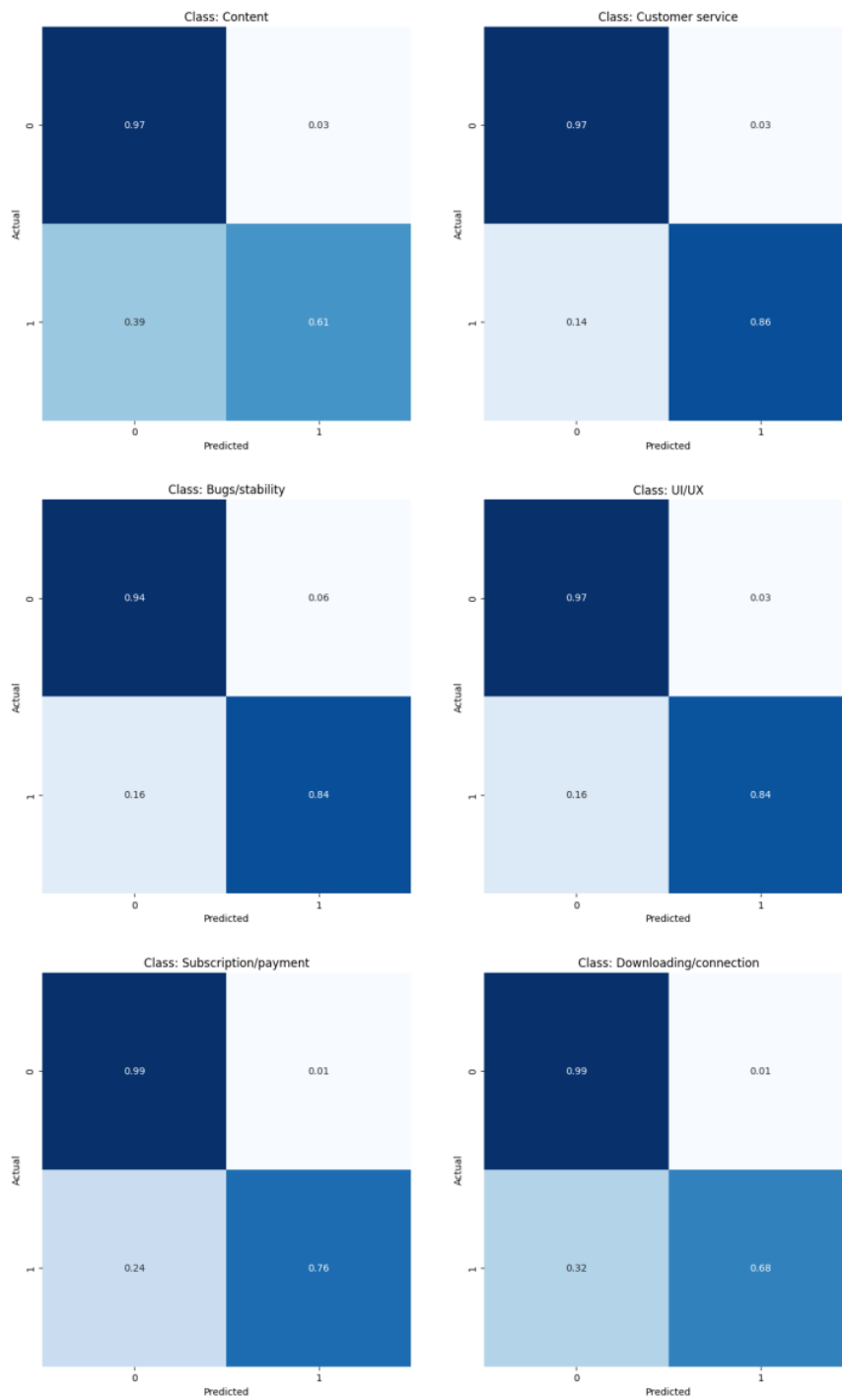
Figure 7.2 Confusion Matrix of GPT 3.5-1106
