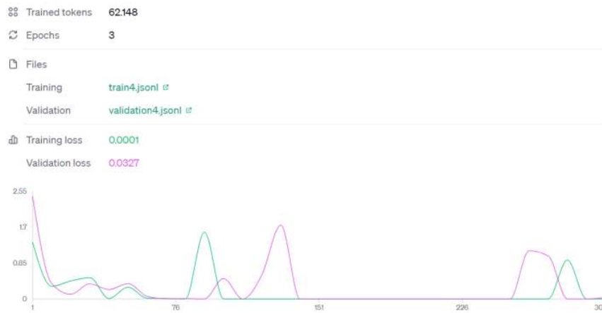
Figure 6.1 GPT-3.5 Turbo 0613 Learning Curve
