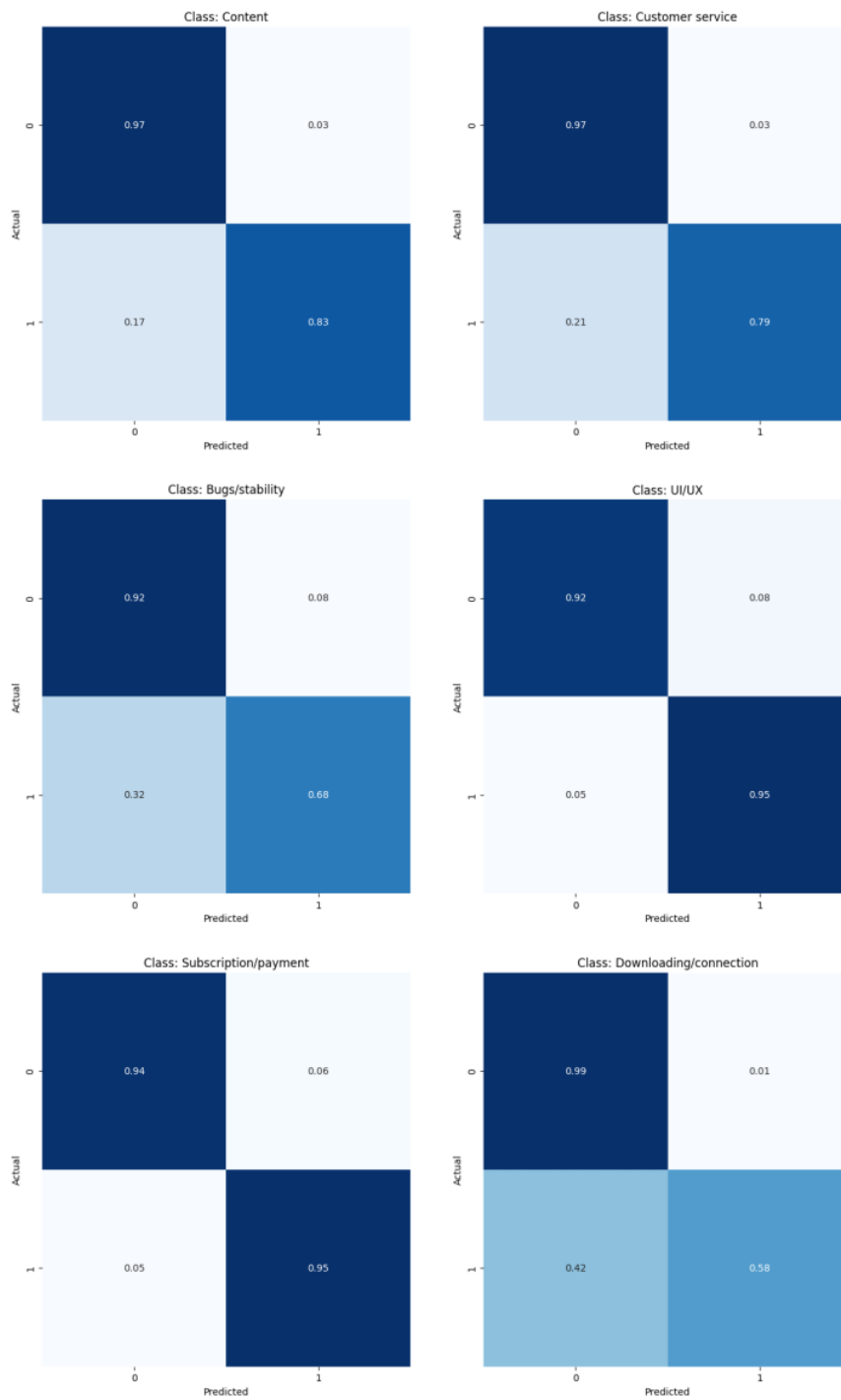
Figure 7.1 Confusion Matrix of GPT 3.5-0613
