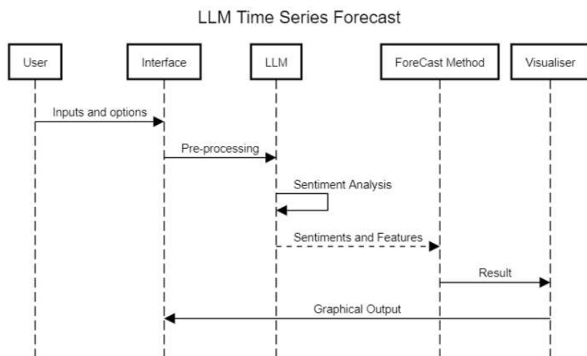
Figure 5.1 Sequence diagram
