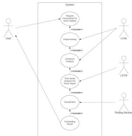
Figure 4.1 Use case diagram
